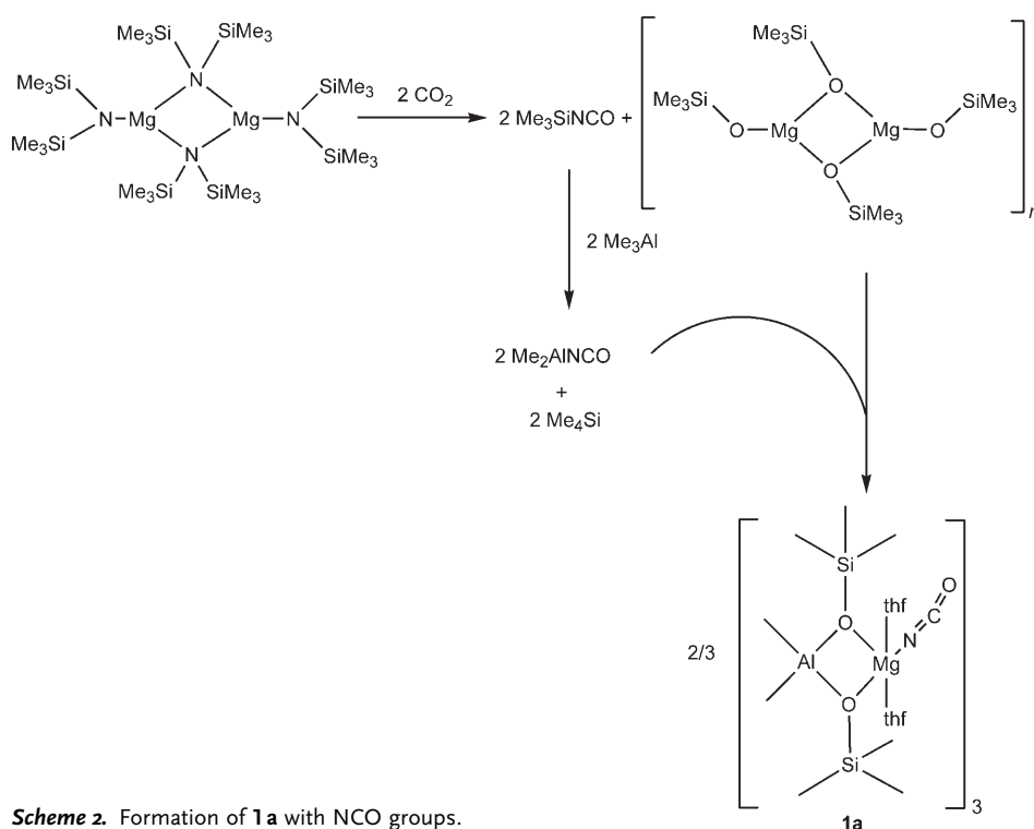
Scheme 2. Formation of 1a with NCO groups.
