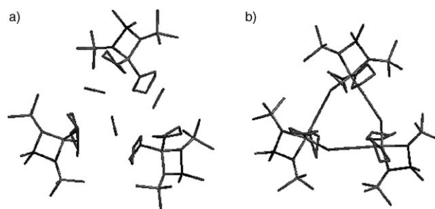
Figure 1. a) Partially optimized structure of 1a ; [7] CO 2 units are dissociating. b) Optimized structure of 1a with N and O atoms exchanged.
